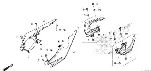
C-24.1 Tampa Lateral (CG160EDA/EDF)
